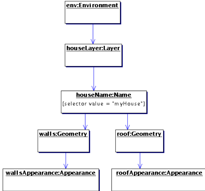
Figure 2: UML instance diagram of a scene graph with a Name element giving the collective name "myHouse" to Geometry elements which model the roof and walls of a house.
